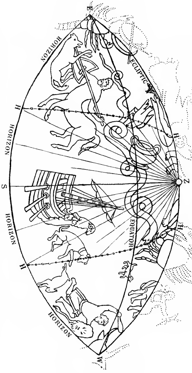
Portion of Sun at Summer Solstice, 3,000 B.C. Observer in Lat. 23° N.
